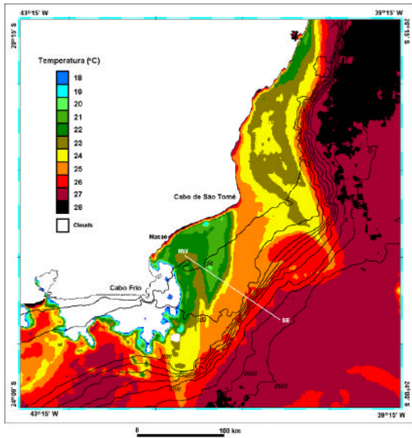
Fig. 2: Sea Surface Temperature (SST) map derived from AVHRR/NOAA-12 image.
