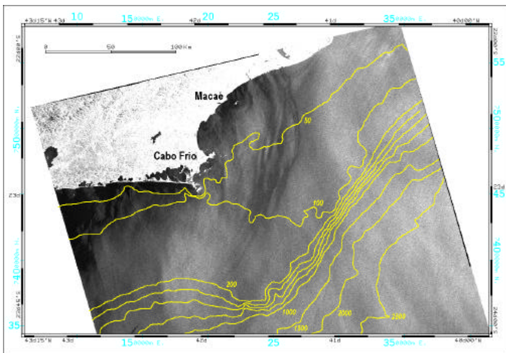
Fig. 4: RADARSAT-1 SCN1 image with bathymetry (meters) offshore Cabo Frio and Macaé.
