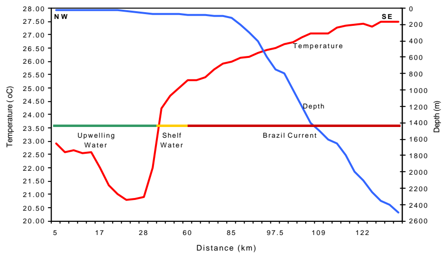
Fig. 3: Macaé profile (see Fig. 2 for location) showing the horizontal variation of sea surface temperature.
