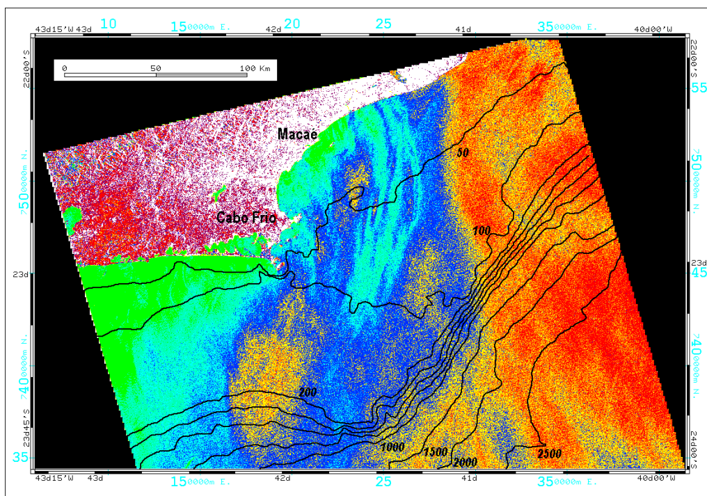
Fig. 5: USTC-classified image with bathymetry (meters) offshore Cabo Frio and Macaé.
