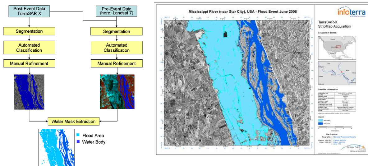
Figure 5. Work flow and resulting flood extent map based on TerraSAR-X (post event) and Landsat ETM (pre event). Dark blue areas are water bodies; light blue depicts flooded areas.
