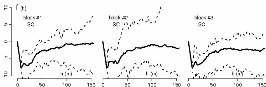
Figure 4: K-functions of final model in all three sample blocks. Solid lines correspond to empirical K-functions, dotted lines are confidence intervals from Monte-Carlo simulation \alpha = 0.1 , n = 20 ), given the fitted soft-core model (SC). All functions are transformed for display purposes by the theoretical K-function under CSR to L = \sqrt{K_{CSR}}/\pi - h .
