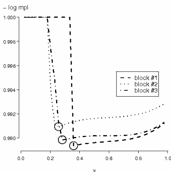
Figure 2: Fitting of a soft-core model to the observed point patterns in sample blocks #1-3. Displayed are the negative log-pseudolikelihood (mpl) curves for different parametrizations
