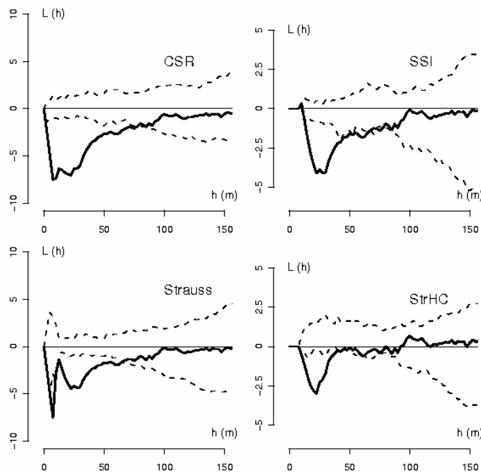
Figure 3: K-functions of sample block #1 for various point process models. Legend: CSR - homogeneous Poisson process, SSI - simple sequential inhibition, Strauss - homogeneous Strauss process, and StrHC - Strauss hard-core. All functions are transformed by the theoretical K-functions of their respective processes to L = K^{-1} - h , e.g. L_{\text{CSR}} = \sqrt{K_{\text{CSR}}/\pi} - h . The bold solid lines are the empirical K-functions, the solid (non-bold), horizontal line is the theoretical K-function, and the dotted lines correspond to the confidence intervals from Monte-Carlo simulation ( \alpha = 0.1 , n = 20 ), given the fitted models.
