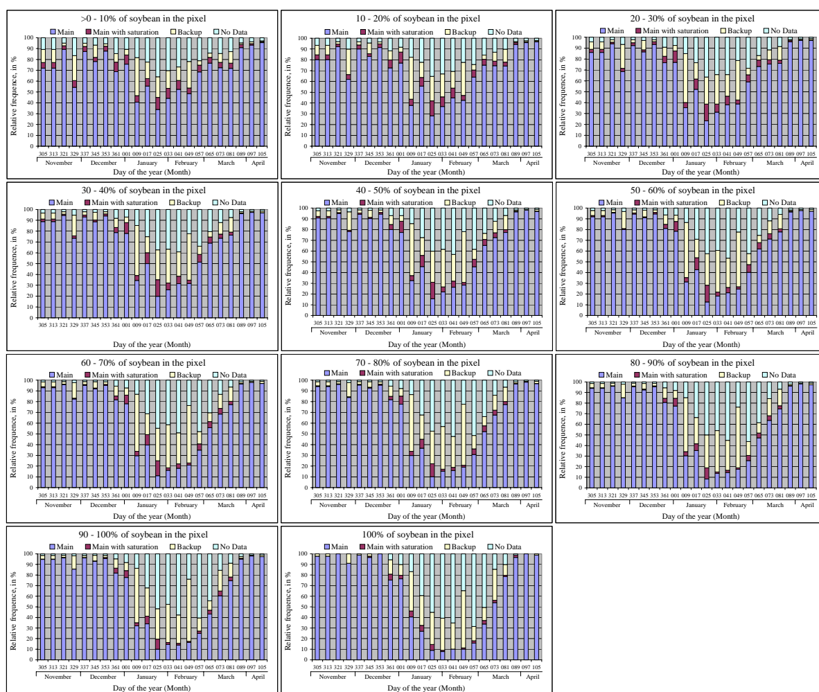
Figure 4: Relative frequency of algorithms (%) in relation to the percentage of soybean percentage in the pixels.
