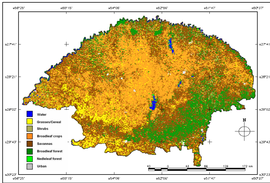
Figure 2: 1 km six-biome landcover map (MOD12Q1) used by the Collection 4 MODIS LAI algorithms.
