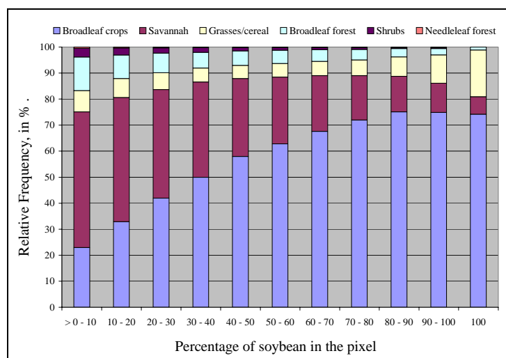
Figure 5: Relative frequency (%) of biome-type by percentage of soybean in the pixel.
