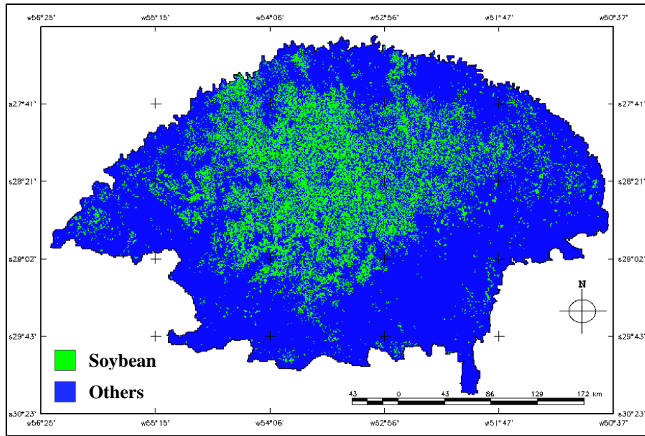
Figure 1: Thematic map of soybean areas mapped over multitemporal Landsat images (Rizzi, 2004).
