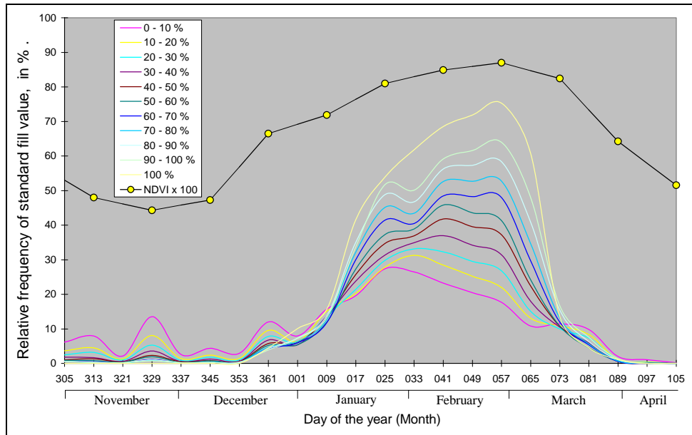
Figure 3: Relative frequency of Standard fill value 255 pixels (%) in relation to the percentage of soybean in the pixel plus the averaged soybean NDVI temporal behavior.
