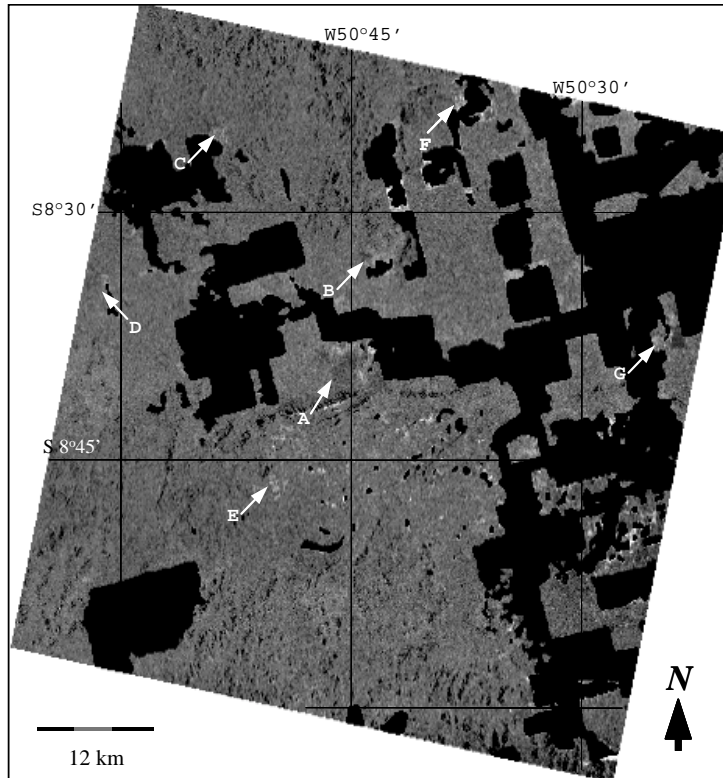
Figure 3. JERS-1 SAR NDI image [1993(March) – 1994(October)] indicating in bright shades areas deforested over the period. Black mask covers areas deforested up to July 1993. Letters refer to areas discussed in the text.
