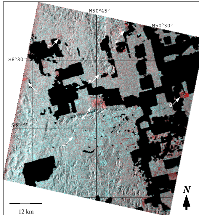
Figure 6. JERS-1 SAR false-color composite [October 1994(R)+October 1996(GB)]. Black mask covers areas deforested up to July 1993. Letters refer to areas discussed in the text.
