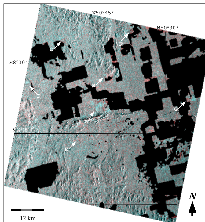
Figure 5. JERS-1 SAR false-color composite [March 1993(R)+October 1994(GB)]. Black mask covers areas deforested up to July 1993. Letters refer to areas discussed in the text.
