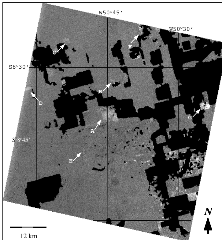
Figure 4. JERS-1 SAR NDI image [1994(October) – 1996(October)] indicating in bright shades areas deforested over the period. Black mask covers areas deforested up to July 1993. Letters refer to areas discussed in the text.
