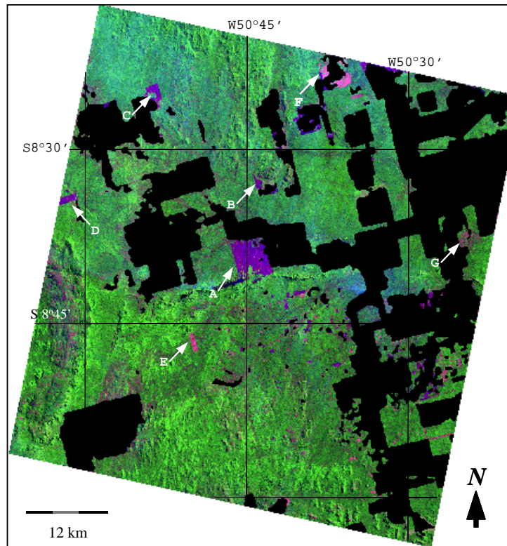
Figure 2. Deforested areas (arrows) indicated in the Landsat-5 TM color composite (TM3B+TM4G+TM5R) acquired in August 1994. Black mask covers areas deforested up to July 1993. Letters refer to areas discussed in the text.
