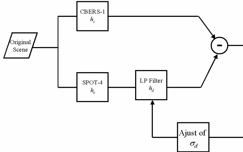
Fig.11 block diagram of low-resolution image simulation
